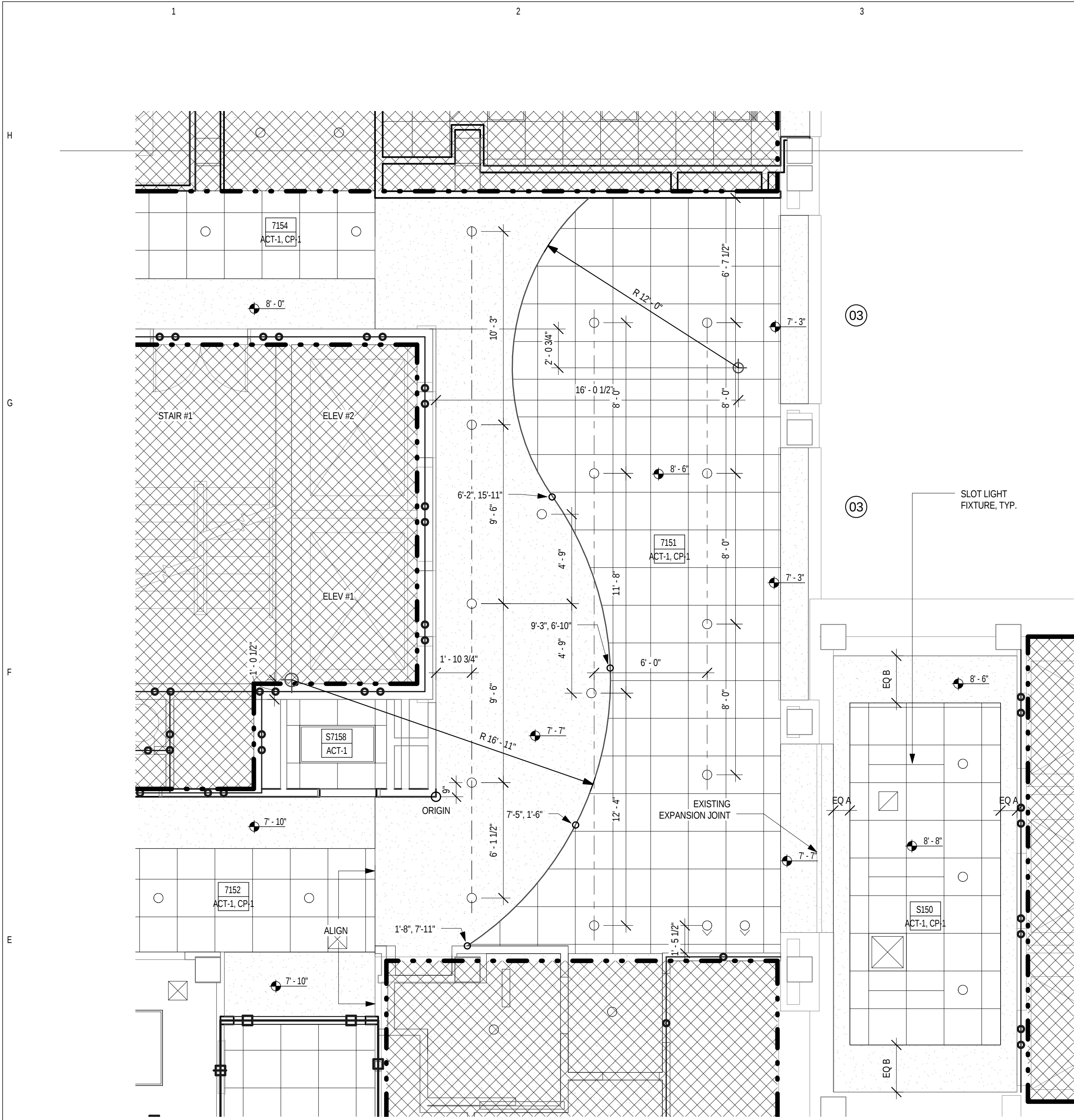
1 REFLECTED CEILING PLAN - LOBBY 1/4" = 1'-0"
