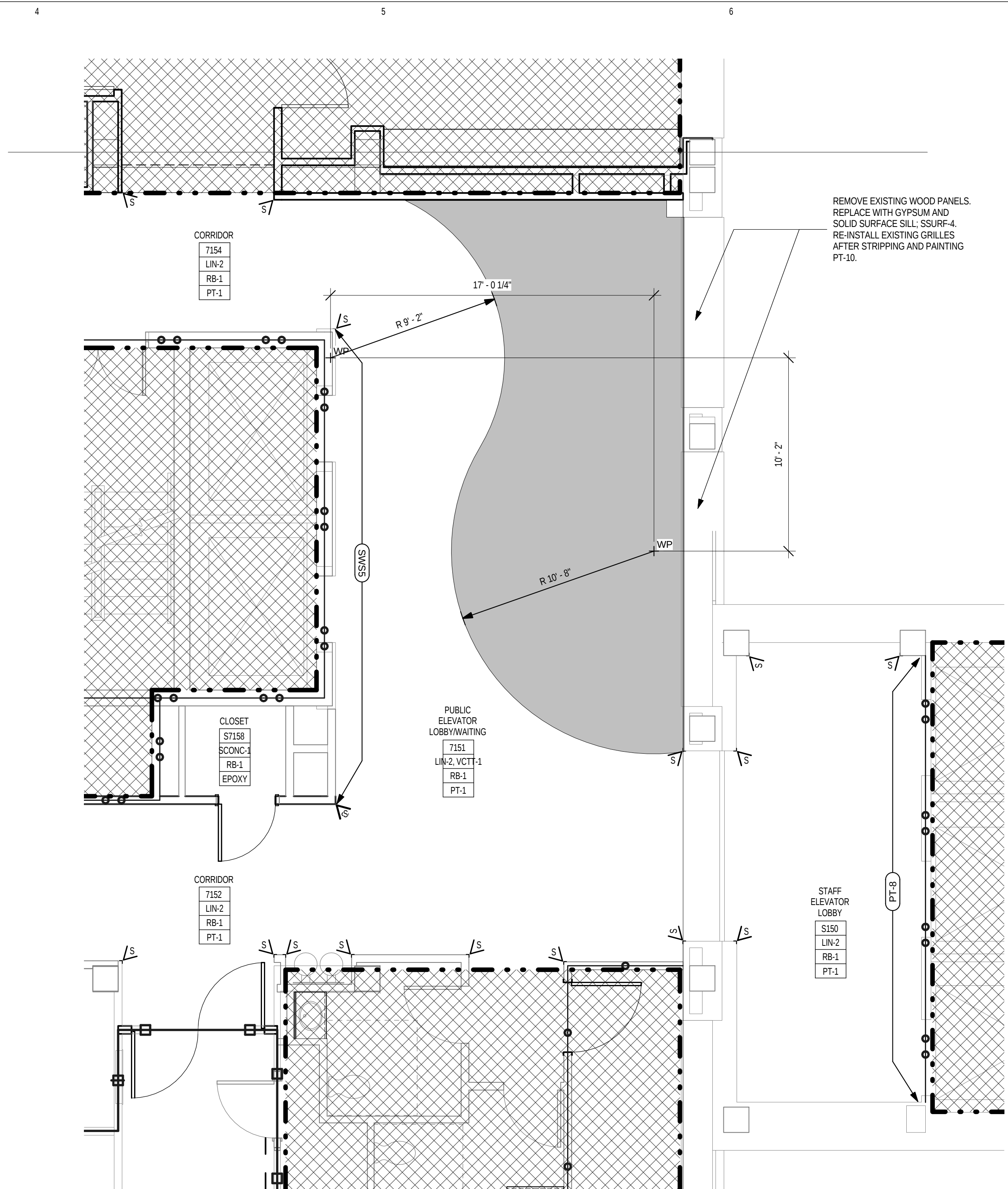
2 NEW WORK & FINISH PLAN - LOBBY 1/4" = 1'-0"
